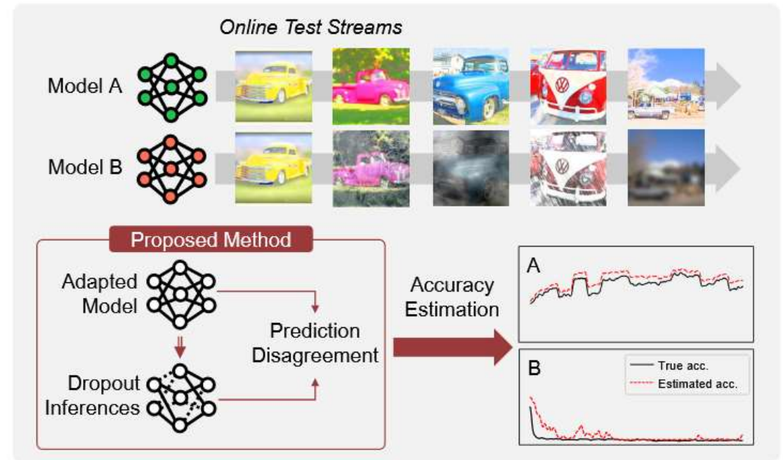
Figure 1. AETTA estimates the model's accuracy after adaptation using unlabeled test data without needing source data or ground-truth labels. AETTA can be integrated into existing TTA methods to estimate their accuracy under various scenarios.
